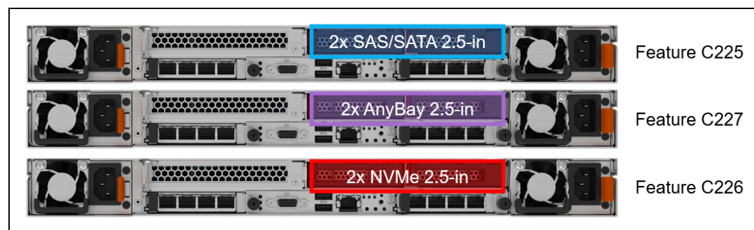
Figure 14. Rear drive bay configurations
