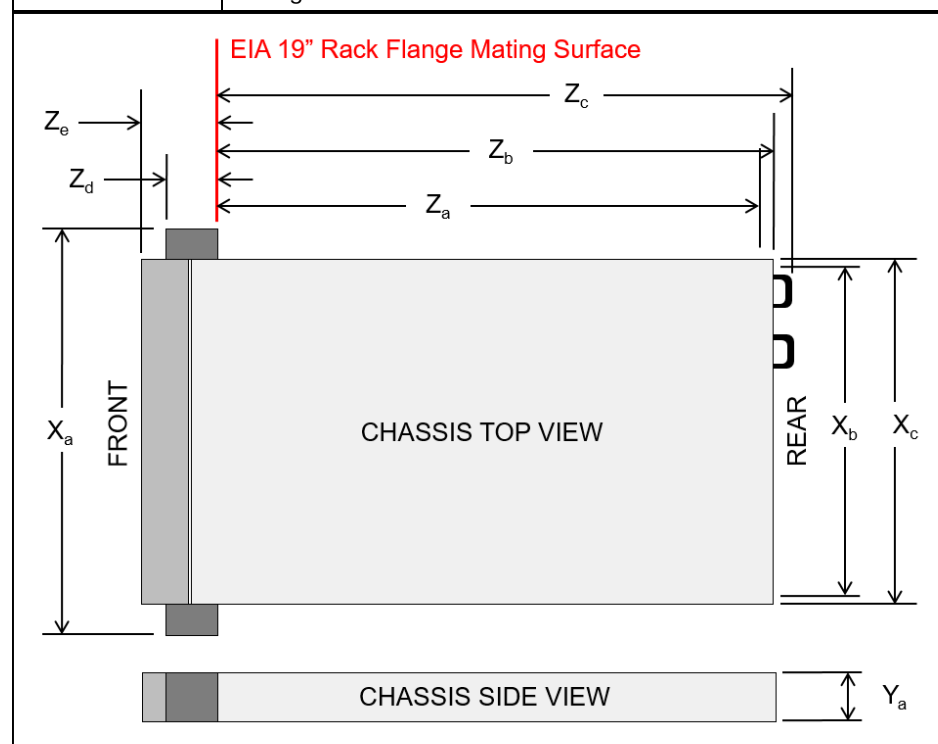
Figure 28. Server dimensions
