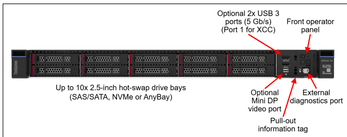
Figure 2. Front view of the SR630 V4 with 2.5-inch drive bays
