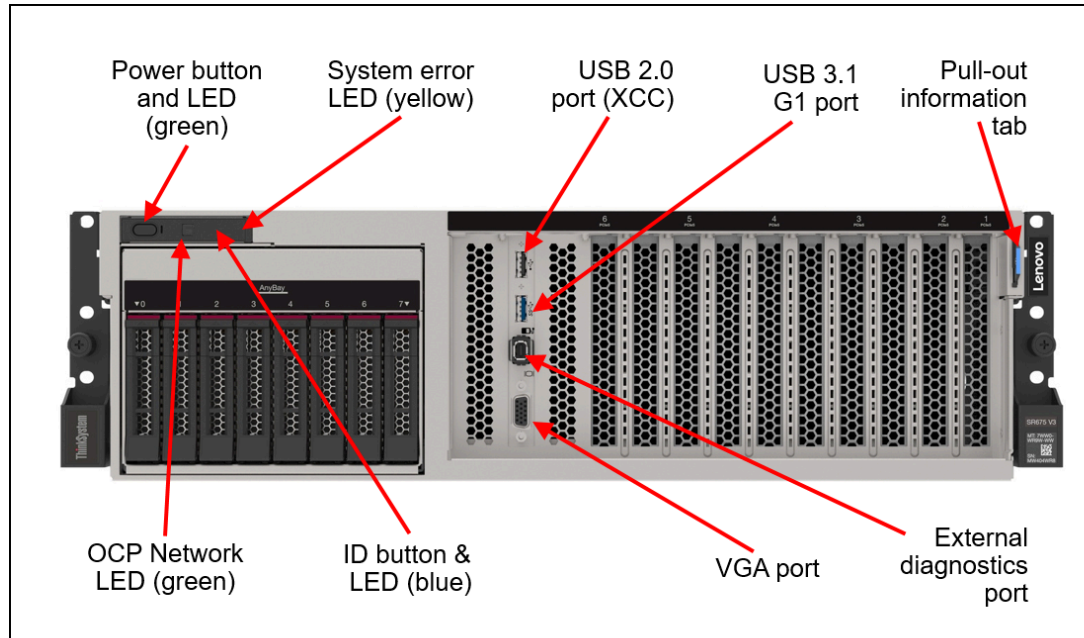
Figure 17. SR675 V3 operator controls
