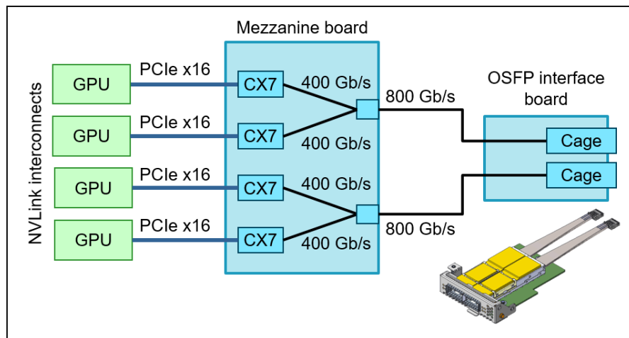
Figure 15. GPU Direct connectivity in the SR675 V3
