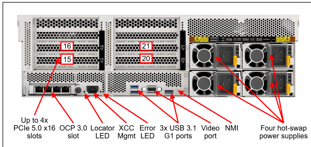
Figure 6. Rear view of the ThinkSystem SR675 V3
