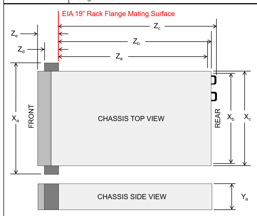
Figure 20. Server dimensions
