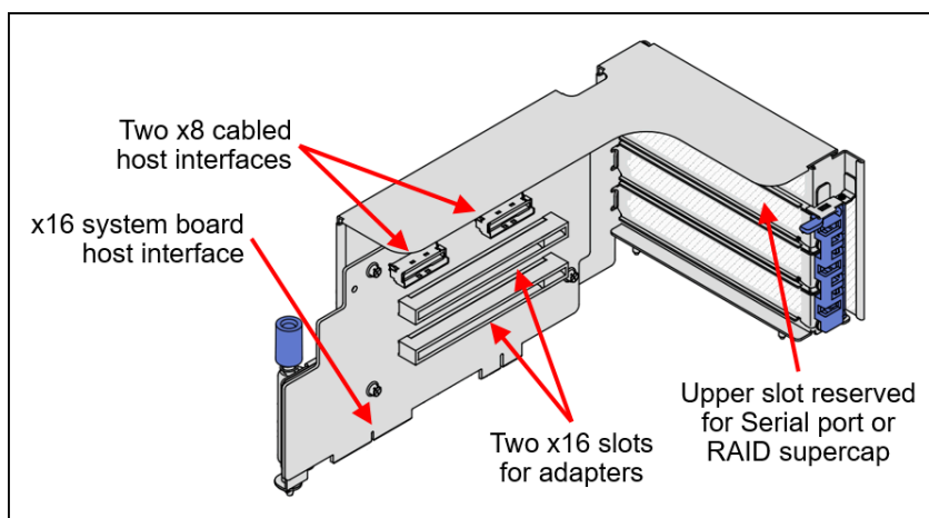
Figure 14. Rear riser
