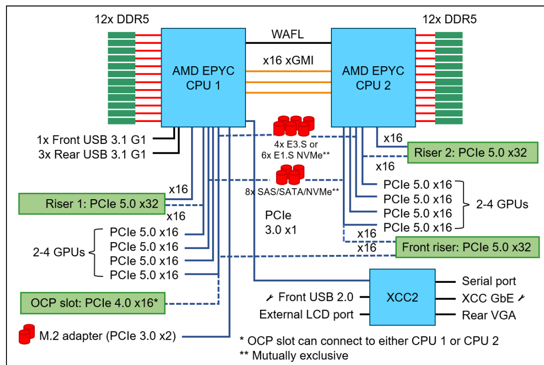
Figure 9. SR675 V3 system architectural block diagram
