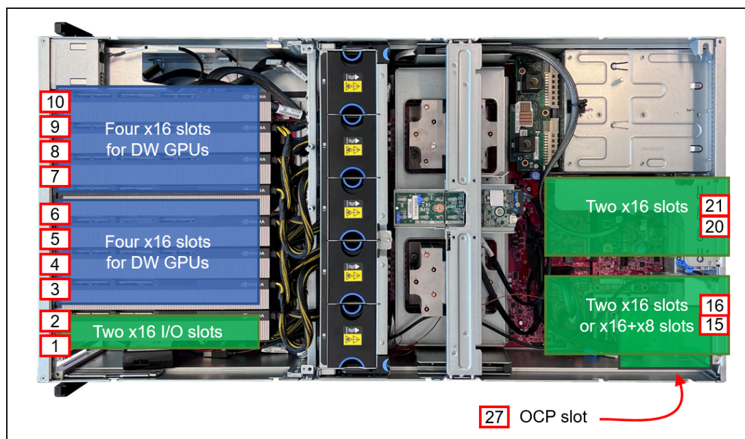
Figure 13. Locations of slots
