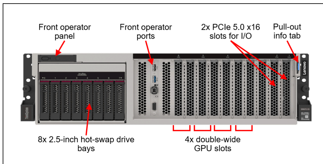
Figure 4. Front view of the SR675 V3 with 4x double-wide PCIe GPUs and 8x 2.5-inch hot-swap drives
