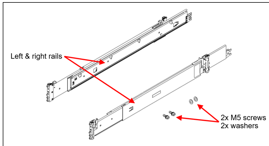
Figure 19. ThinkSystem SR675 V3 Toolless Slide Rail contents
