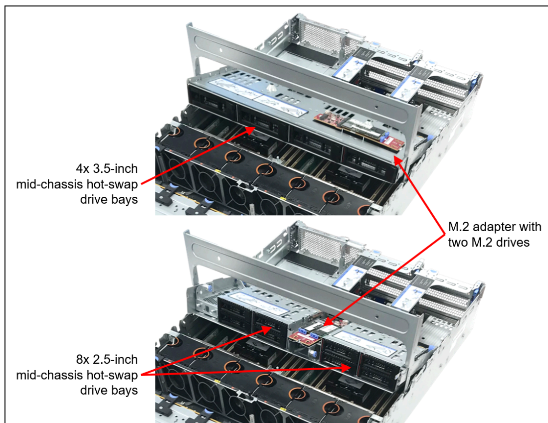
Figure 12. Mid-chassis drive bays
