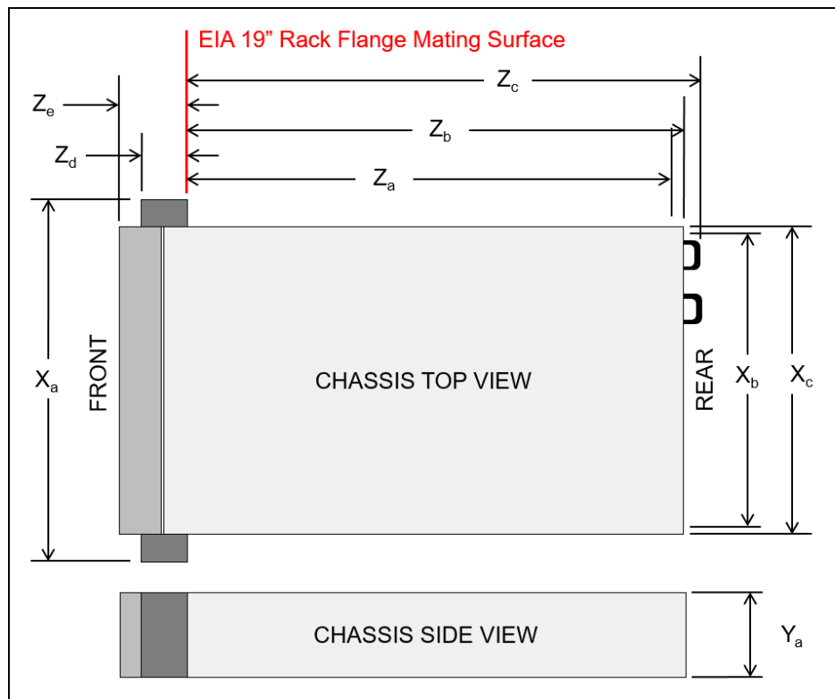
Figure 27. Server dimensions
