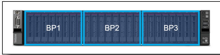
Figure 14. Backplane numbering
